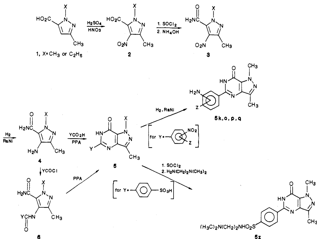
Scheme II
